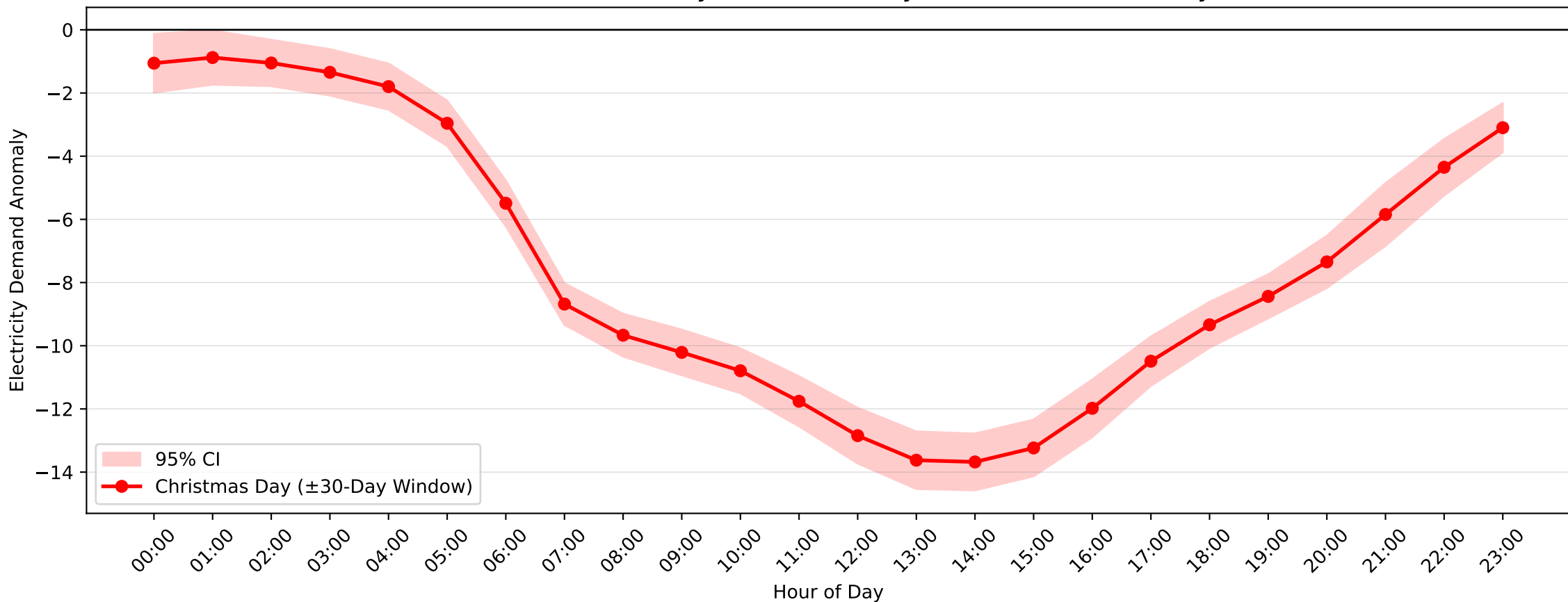
Marrickville Demand Anomaly: Christmas Day (2004–2017, \pm 30 -Day Window)
